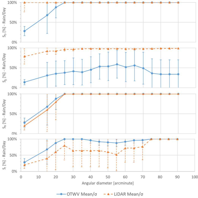
Figure 7. Expected visual task scores and standard deviations \sigma (standard error bars) for OTWV (blue) and LiDAR (red) for the scenario Rain/Day .
