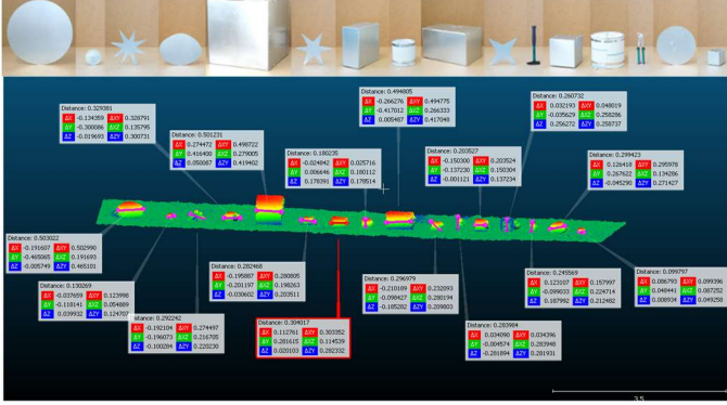
Figure 1. Shown are 16 out of 23 test objects (top row) and corresponding LiDAR point clouds scanned at 20 meters distance (second row) together with the object dimensions. Notice, that the object arrangement differs from the experimental setup depicted in Figure 3.
