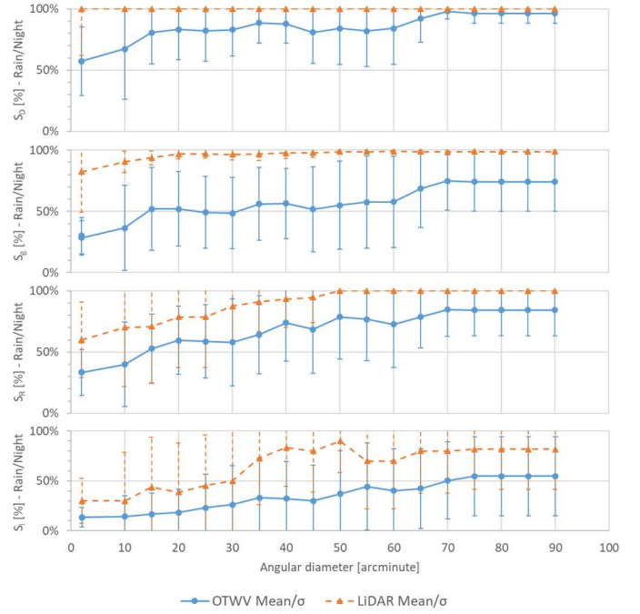
Figure 8. Expected visual task scores and standard deviations \sigma (standard error bars) for OTWV (blue) and LiDAR (red) for the scenario Rain/Night .
