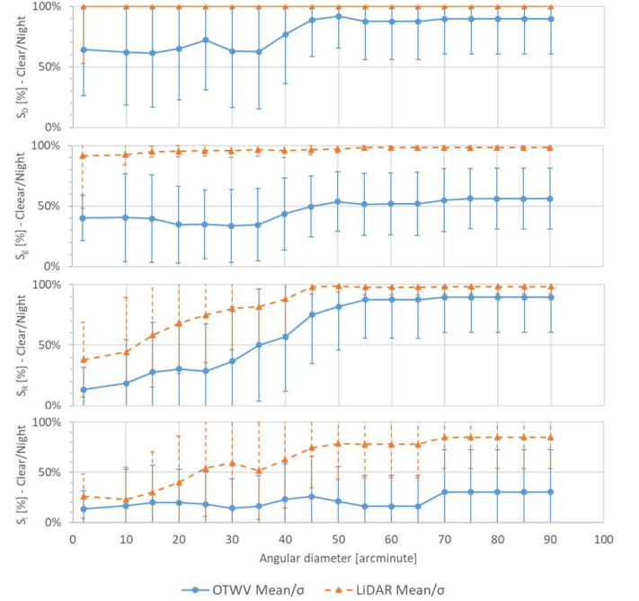
Figure 6. Expected visual task scores and standard deviations \sigma (standard error bars) for OTWV (blue) and LiDAR (red) for the scenario Clear/Night .
