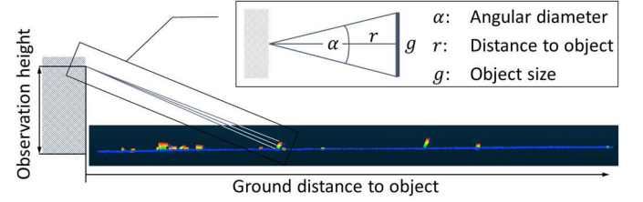
Figure 3. Illustration of the experimental setup. Shown is a side view of the LiDAR point clouds capturing the test objects. The line of sight distance, ground distance and the object size give rise to the angular object size according to (1).
