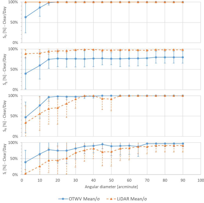
Figure 5. Expected visual task scores and standard deviations \sigma (standard error bars) for OTWV (blue) and LiDAR (red) for the scenario Clear/Day .
