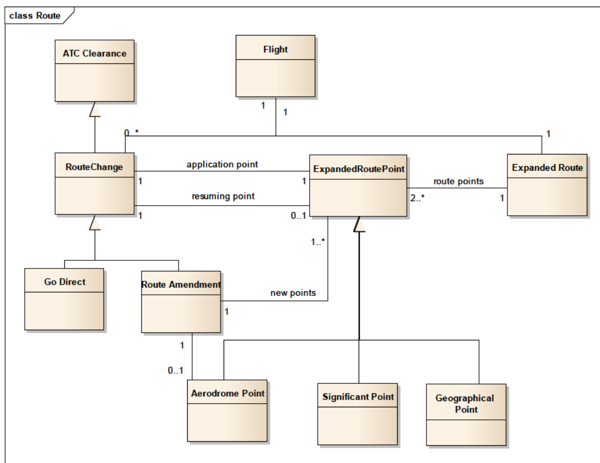
Figure 9: Route Domain
