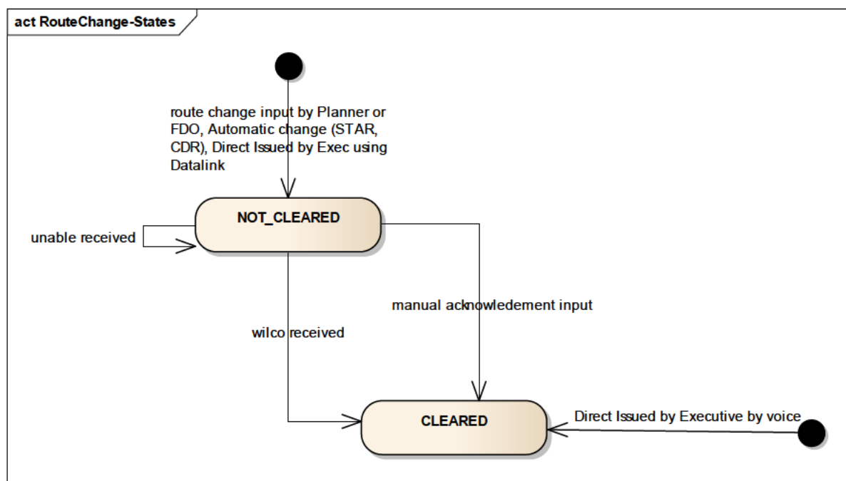
Figure 11 Route Change Operational Status Diagram
