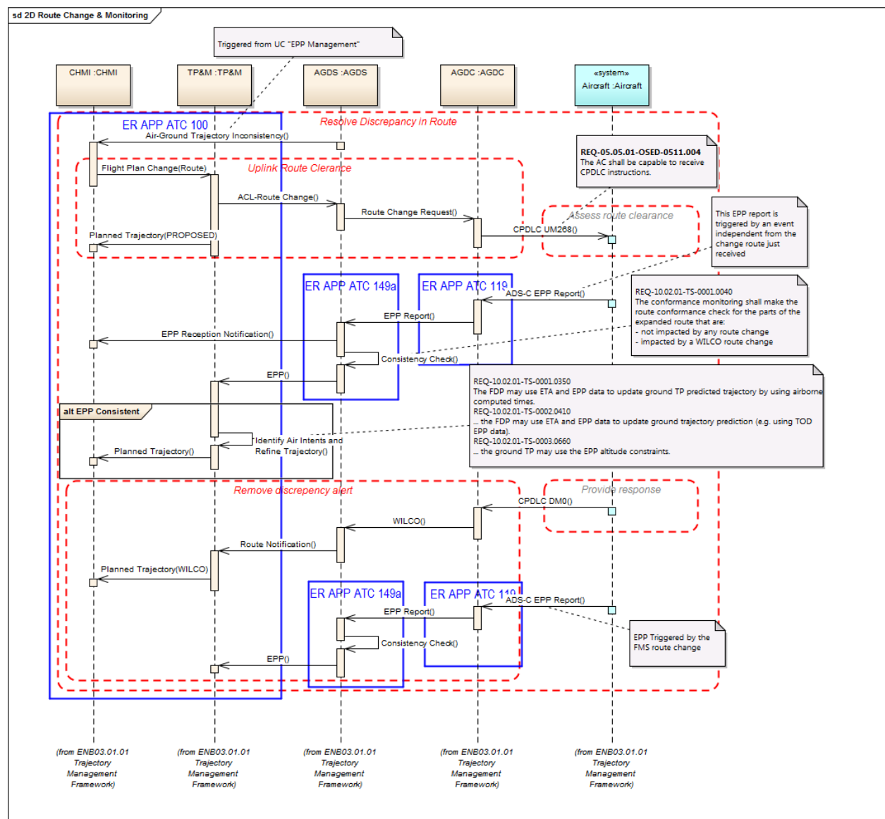
Figure 4 Functional View
