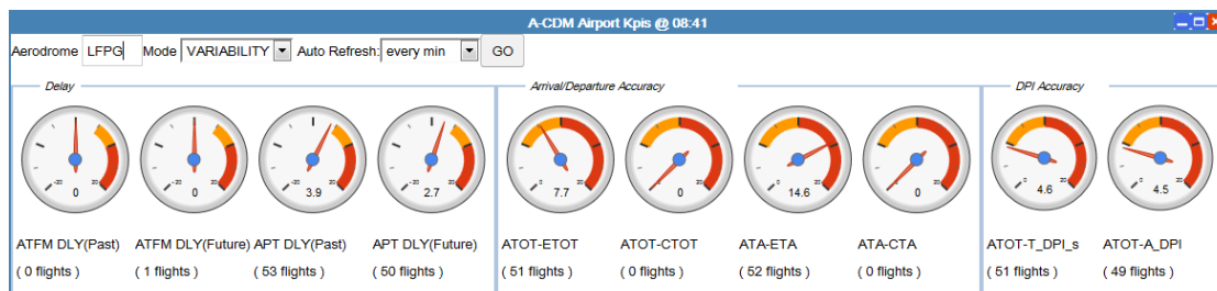
Figure 7 Airport KPIs
